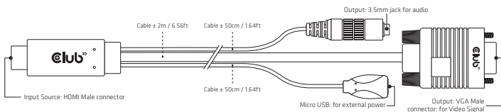
The Club 3D CAC-1712 HDMI™ to VGA Cable provides a 3.5 mm Jack for sound, which is not standard on the VGA port. A Micro USB port is also provide for External Power.
